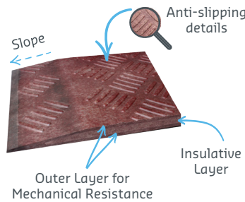
Development of a specific design for each application. Design example for two hours CSP resistance with low thickness 3+9+3 (15mm) - density (700kg/m 3 )
