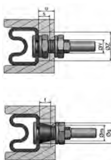
Assembly A
