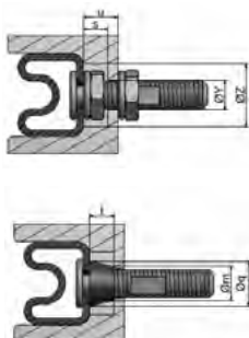
Assembly A
